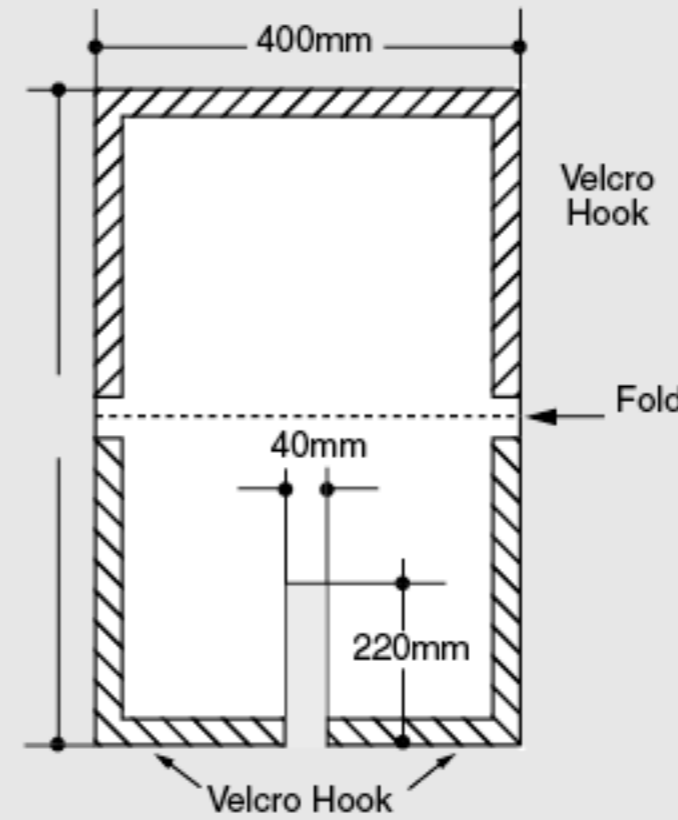
TYPE 3 - D-Iron Assembly Cover
