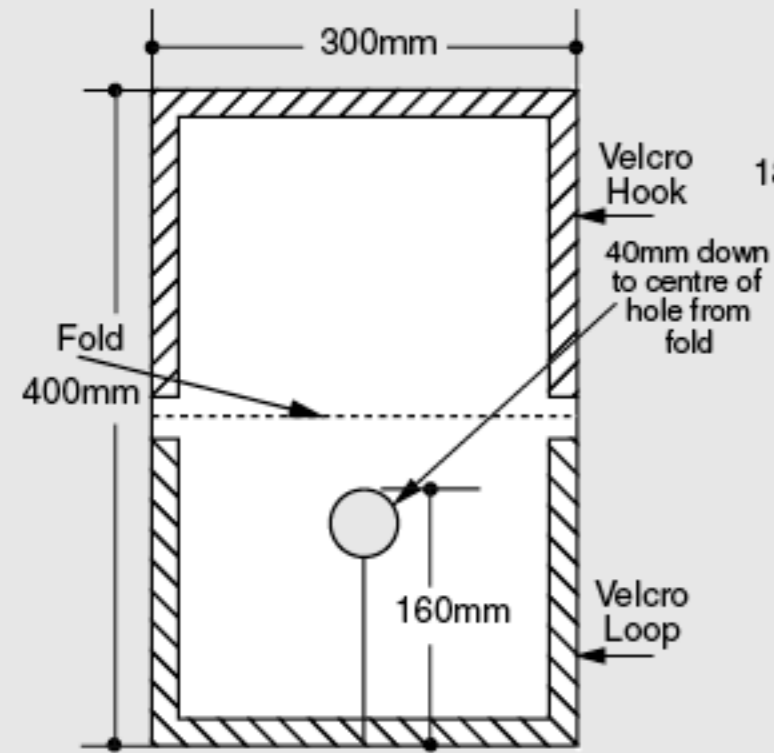
TYPE 1 - Reel Insulator Cover
