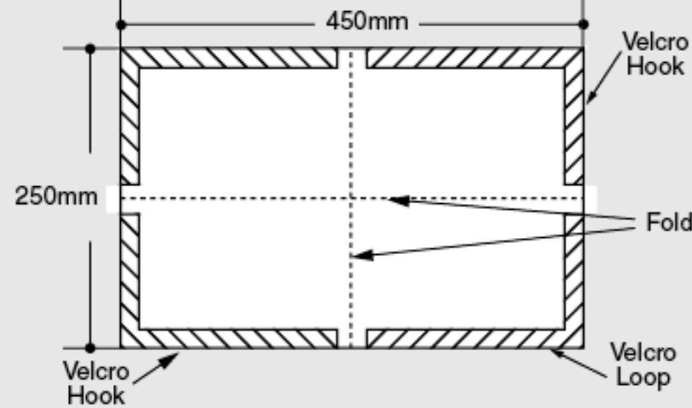
TYPE 5 - General Purpose Cover
