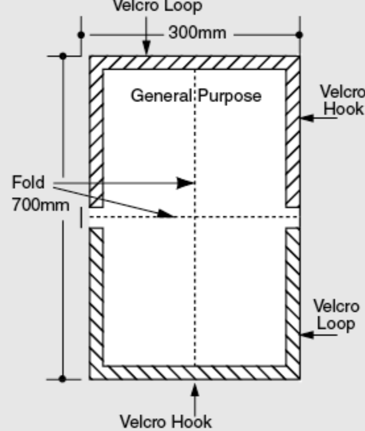
TYPE 6 - General Purpose Cover
