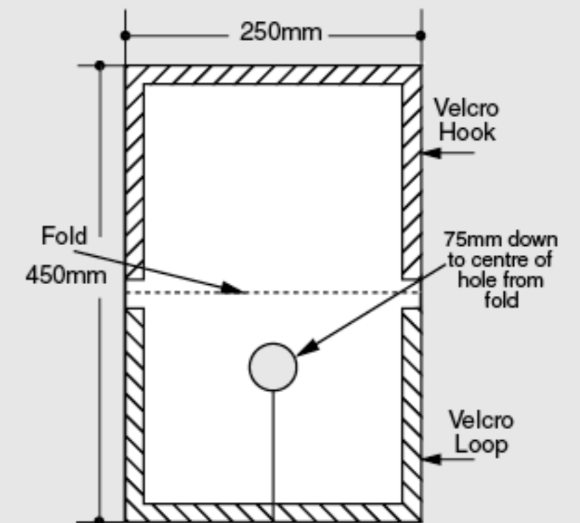
TYPE 7 - Key Hole Cover
